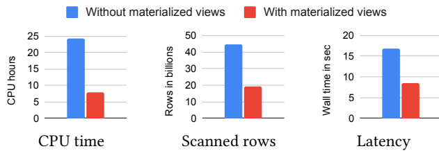
Figure 4: Subquery optimization with materialized views
